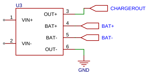
TP4056 Charging Module
