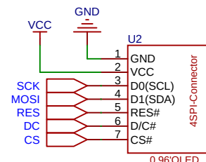
7Pin_SPI_OLED
